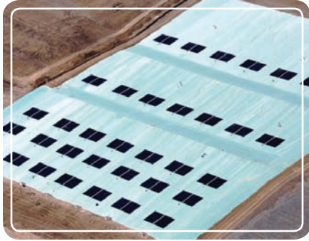
The nation's first Solar Energy Cover (above) is in place on our Tessman Road Landfill in San Antonio.
